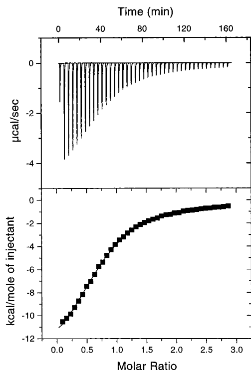
FIGURE 2: Calorimetric titration of W191G with 2AT. Isothermal titration calorimetry profile of W191G titrated with 2AT in 100 mM BIS-TRIS propane at pH 6.0. The upper graph shows the raw data for the heat evolved following each addition of 2AT to the protein in microcalories per second. Shown at the bottom is the corrected integrated area of each peak as a function of molar ratio. The fitted line corresponds to a single-site binding model which gives a K_a of 3.66 \times 10^4 \text{ M}^{-1} , 0.8 molecule of 2AT bound per site, and a \Delta H of -15.2 \text{ kcal/mol} .
